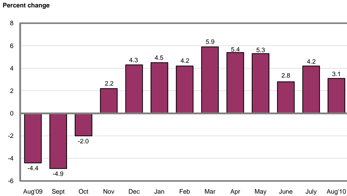
Chart 2. 12-month percent changes in the Producer Price Index for Finished Goods, not seasonally adjusted: August 2009 – August 2010
