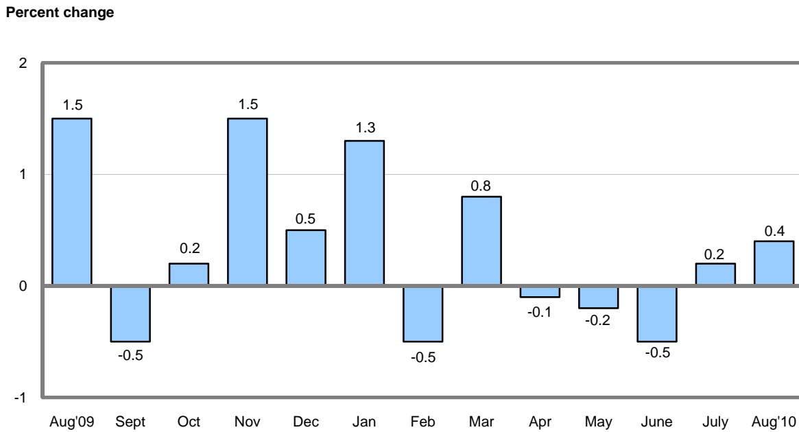
Chart 1. Monthly percent changes in the Producer Price Index for Finished Goods, seasonally adjusted: August 2009 – August 2010
