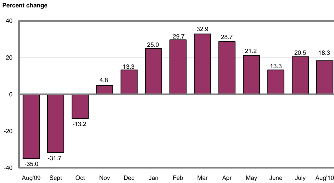
Chart 6. 12-month percent changes in the Producer Price Index for Crude Materials, not seasonally adjusted: August 2009 – August 2010
