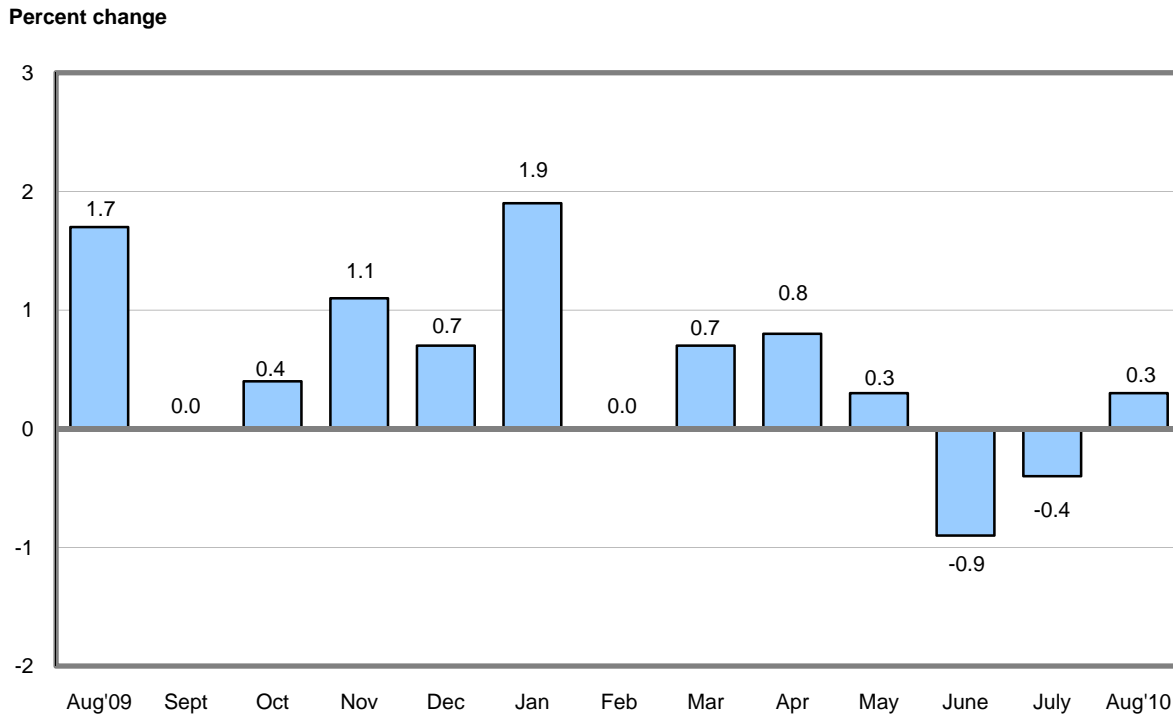
Chart 3. Monthly percent changes in the Producer Price Index for Intermediate Goods, seasonally adjusted: August 2009 – August 2010
