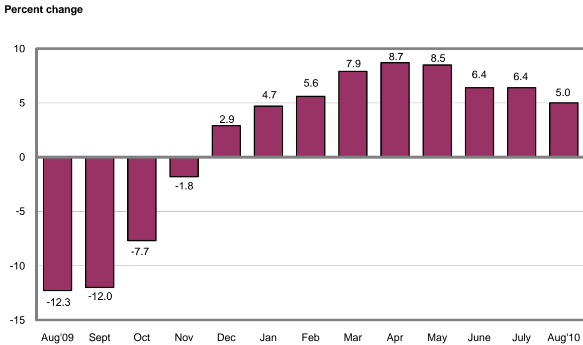
Chart 4. 12-month percent changes in the Producer Price Index for Intermediate Goods, not seasonally adjusted: August 2009 – August 2010
