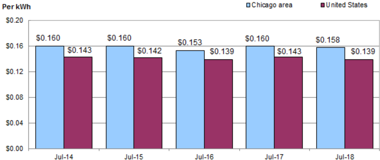
Chart 2. Average prices for electricity, Chicago-Naperville-Elgin and the United States, 2014-2018 (as of July)
