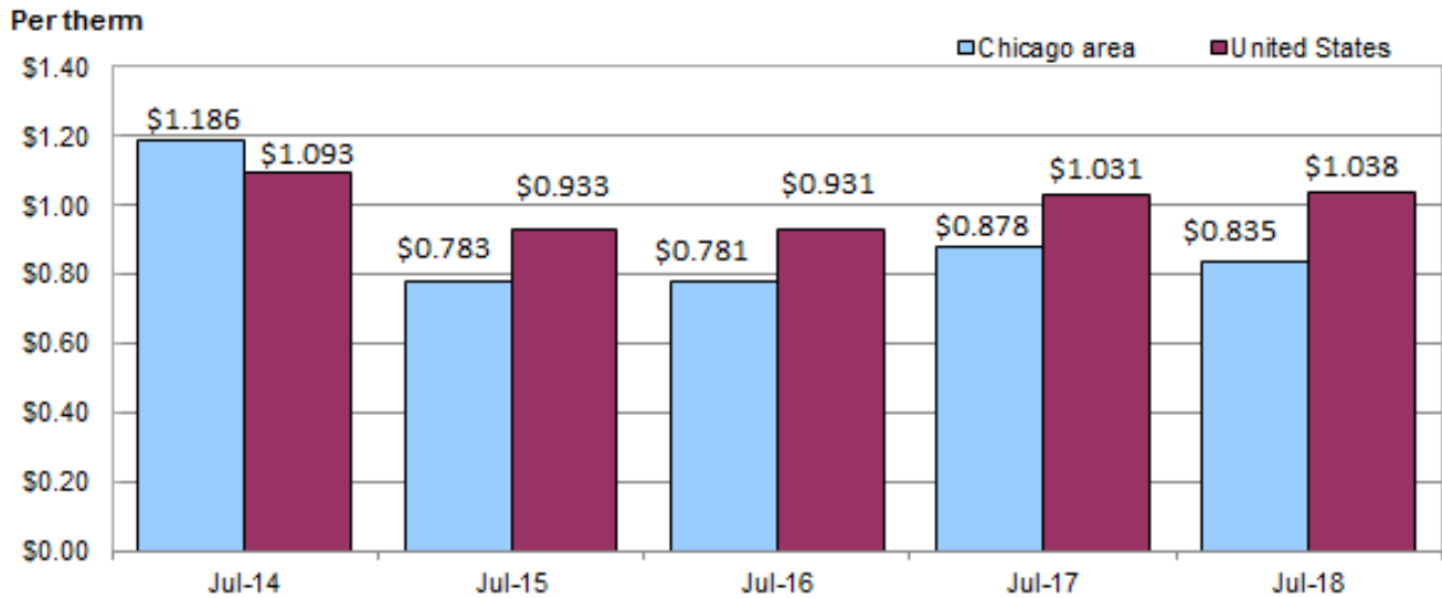
Chart 3. Average prices for utility (piped) gas, Chicago-Naperville-Elgin and the United States, 2014-2018 (as of July)
