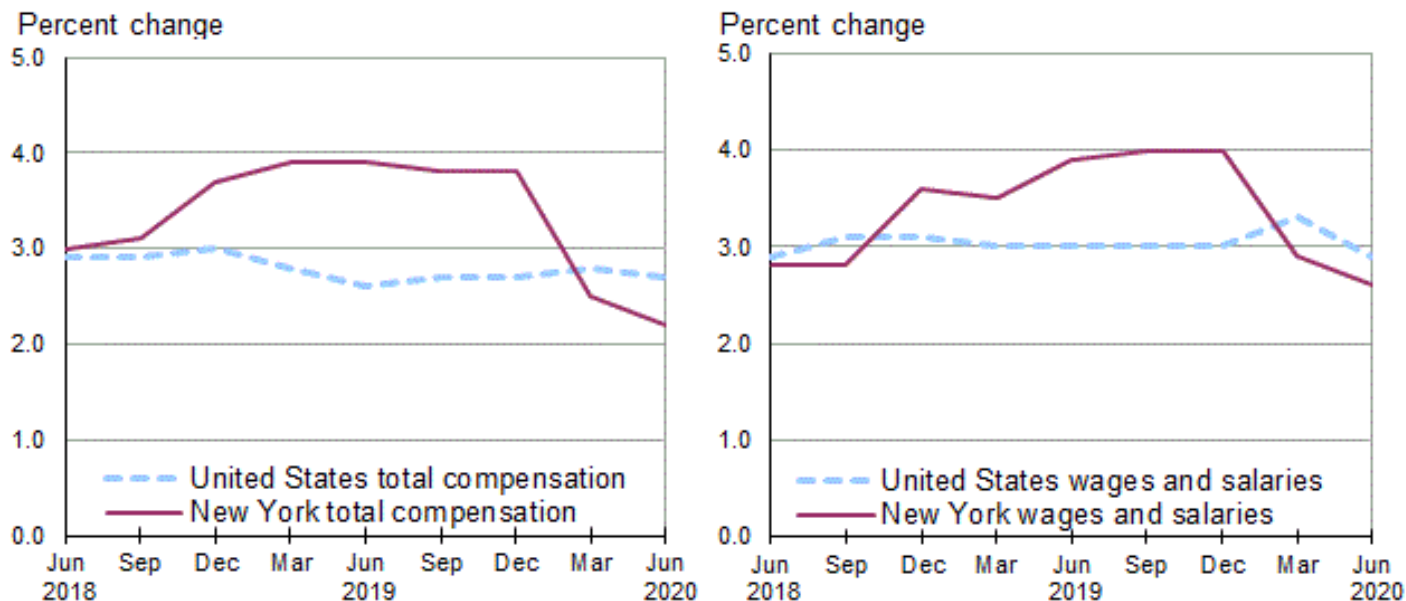
Chart 1. Twelve-month percent changes in the Employment Cost Index, private industry workers, United States and the New York area, not seasonally adjusted, June 2018–June 2020
