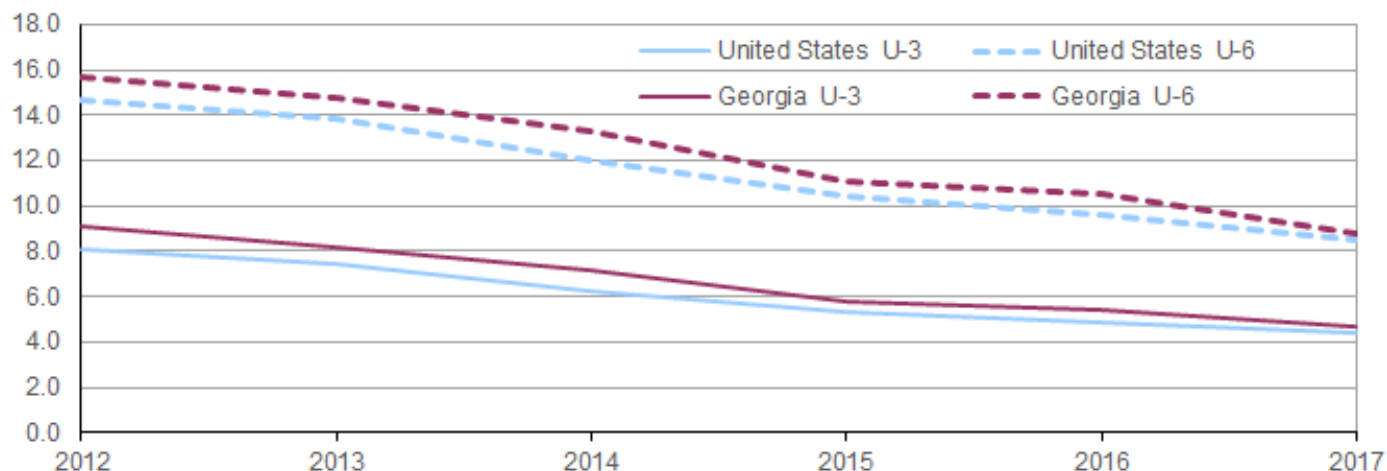
Chart 1. Two alternative measures of labor underutilization, United States and Georgia, 2012–17 annual averages
