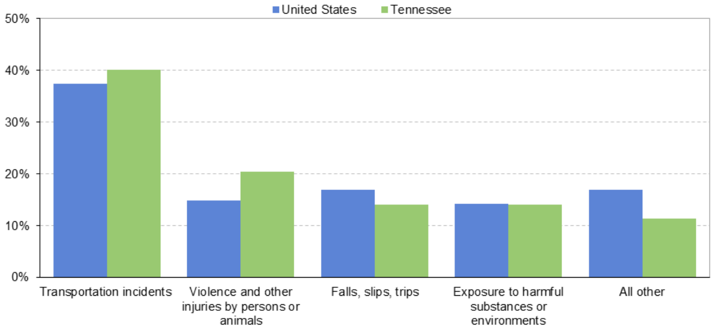
Chart 2. Percent distribution of total fatal occupational injuries by event, United States and Tennessee, 2020
