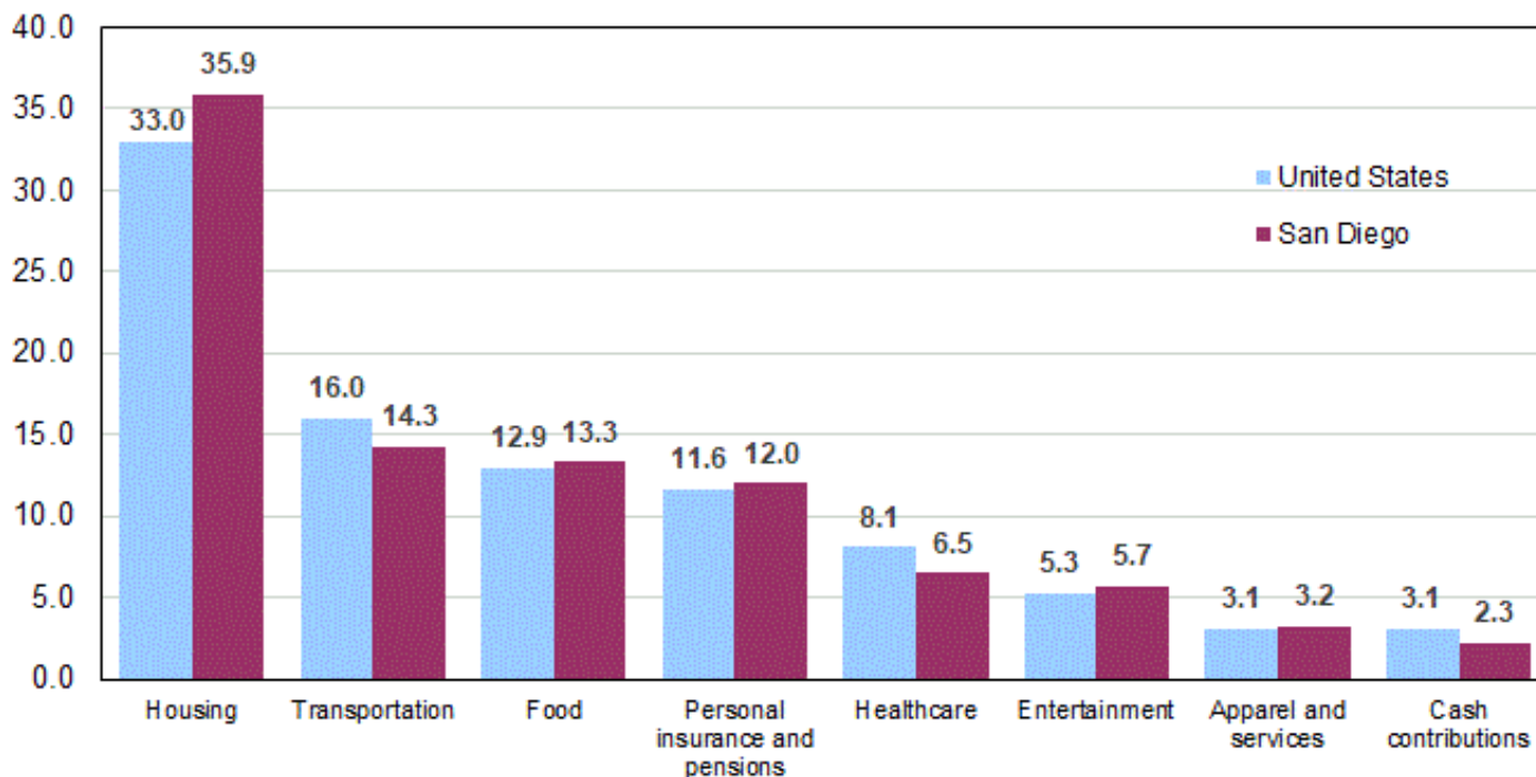
Chart 1. Percent distribution of average annual expenditures for eight major categories in the United States and San Diego metropolitan area, 2017–18
